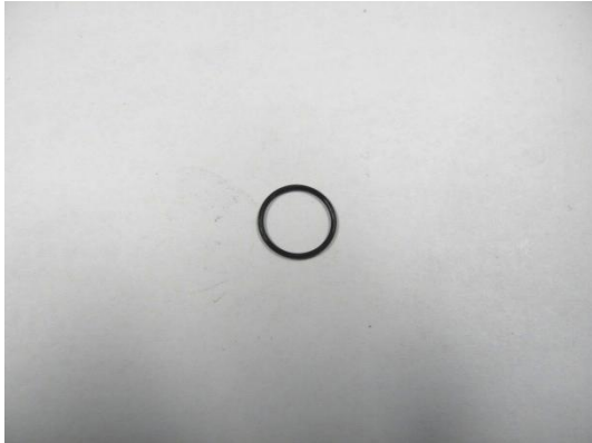
TA004029 O-RING 12.0X 1.0 PERBUNA 76 SH
